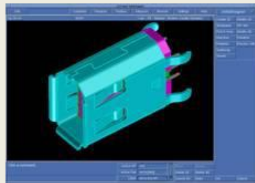
Mold-Flow Analysis
