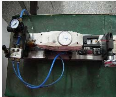
Tensometer
